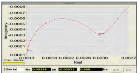
Nyquist diagram
